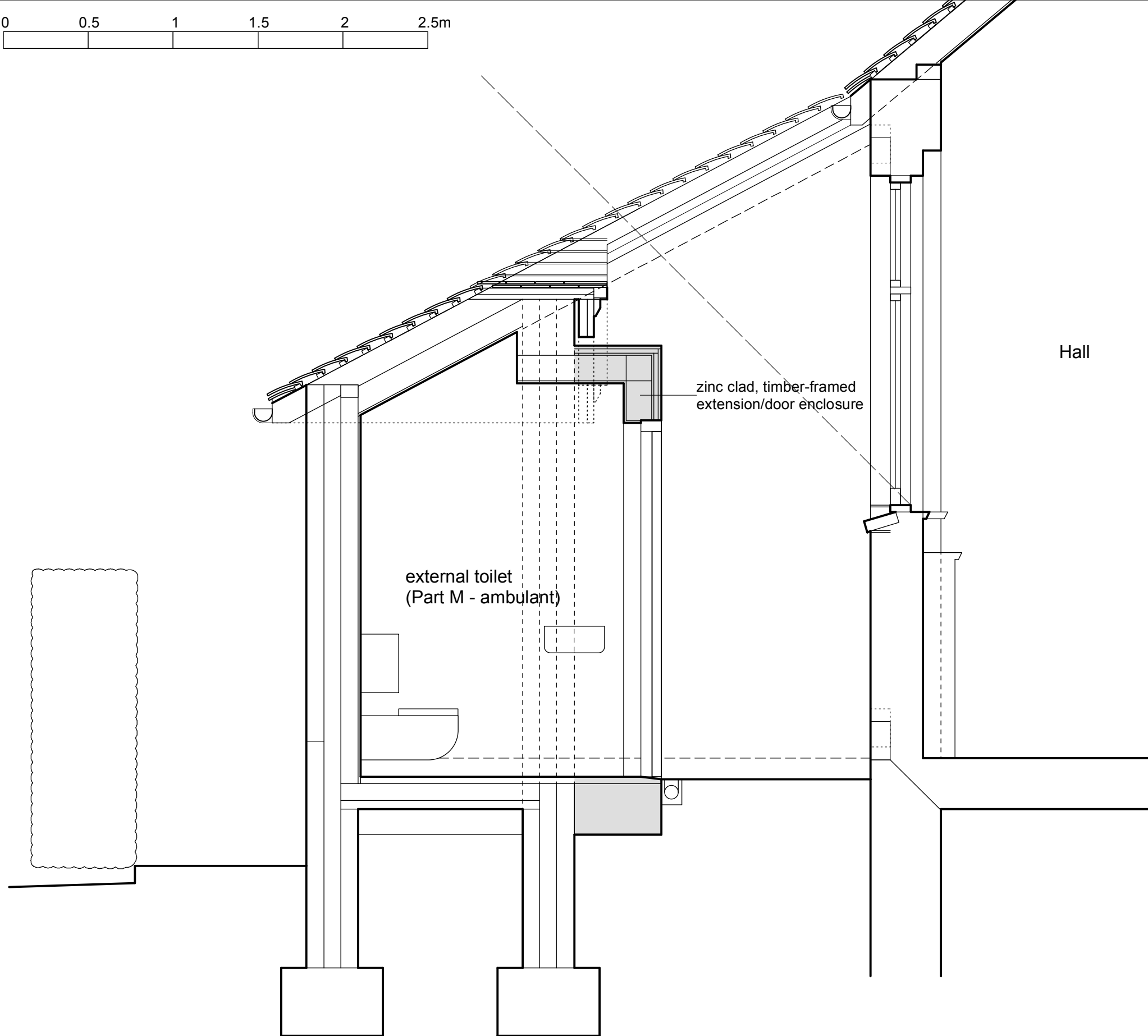
section - option 2 - ambulant wc
